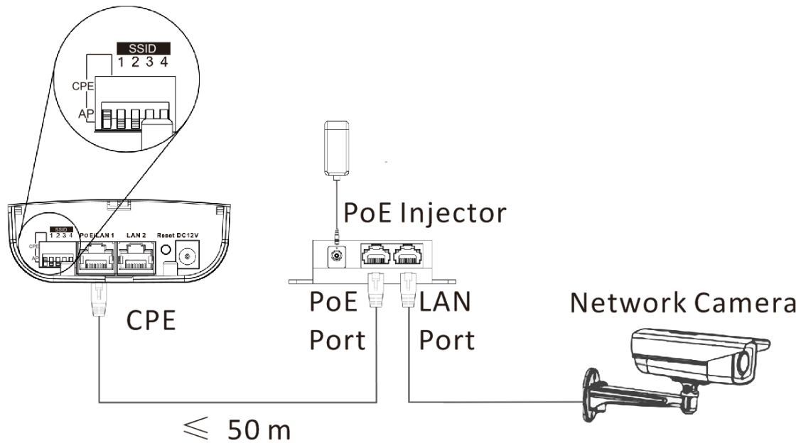
Figure 2-7 CPE Connection
